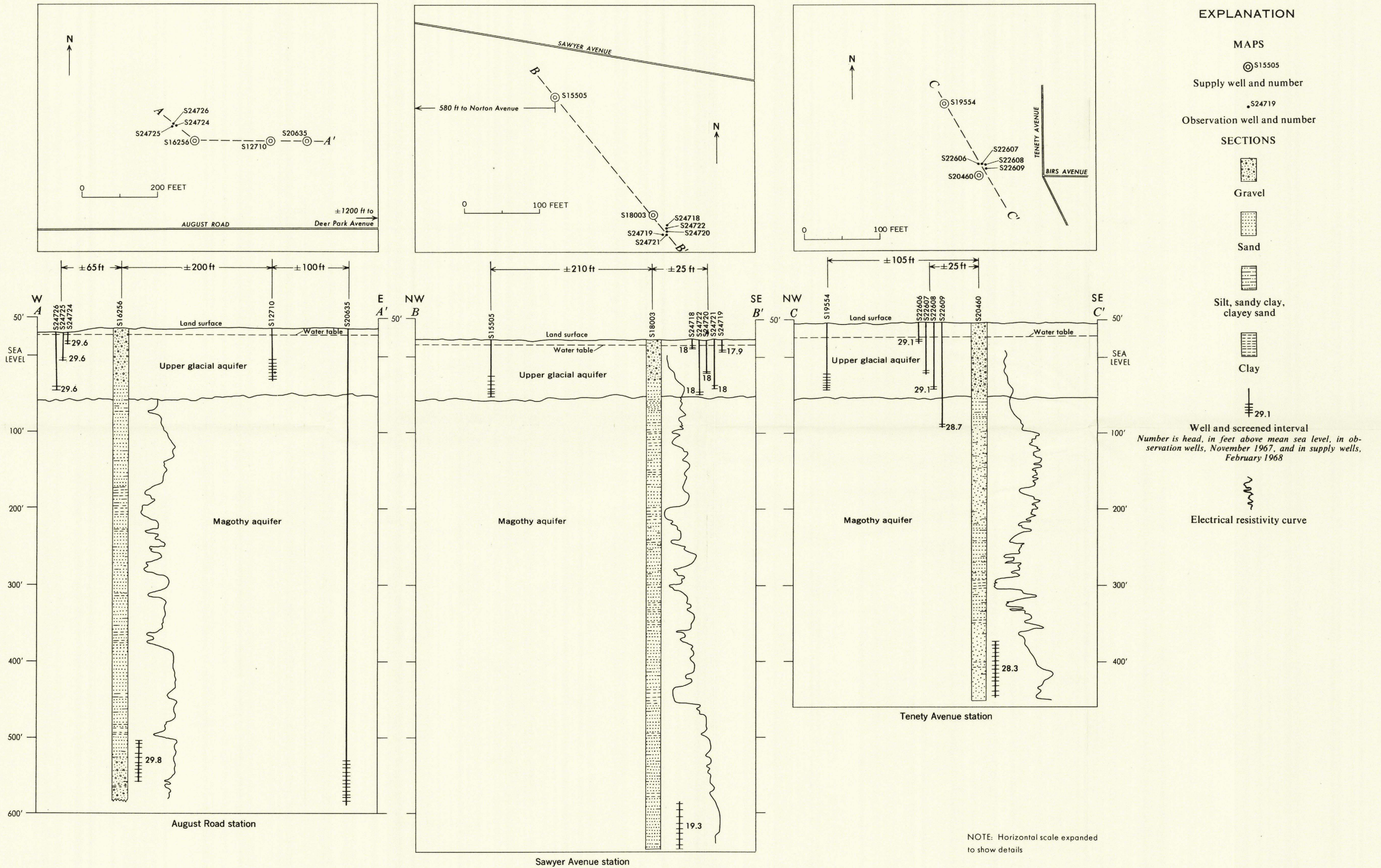
DIAGRAMS SHOWING HYDROGEOLOGIC RELATIONS AT THREE WELL FIELDS IN SOUTHWESTERN SUFFOLK COUNTY, LONG ISLAND, NEW YORK
