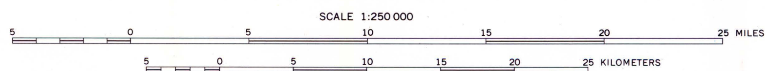
MAPS SHOWING BEDROCK GEOLOGY AND THICKNESS OF GLACIAL DRIFT, MESABI IRON RANGE, NORTHEASTERN MINNESOTA
