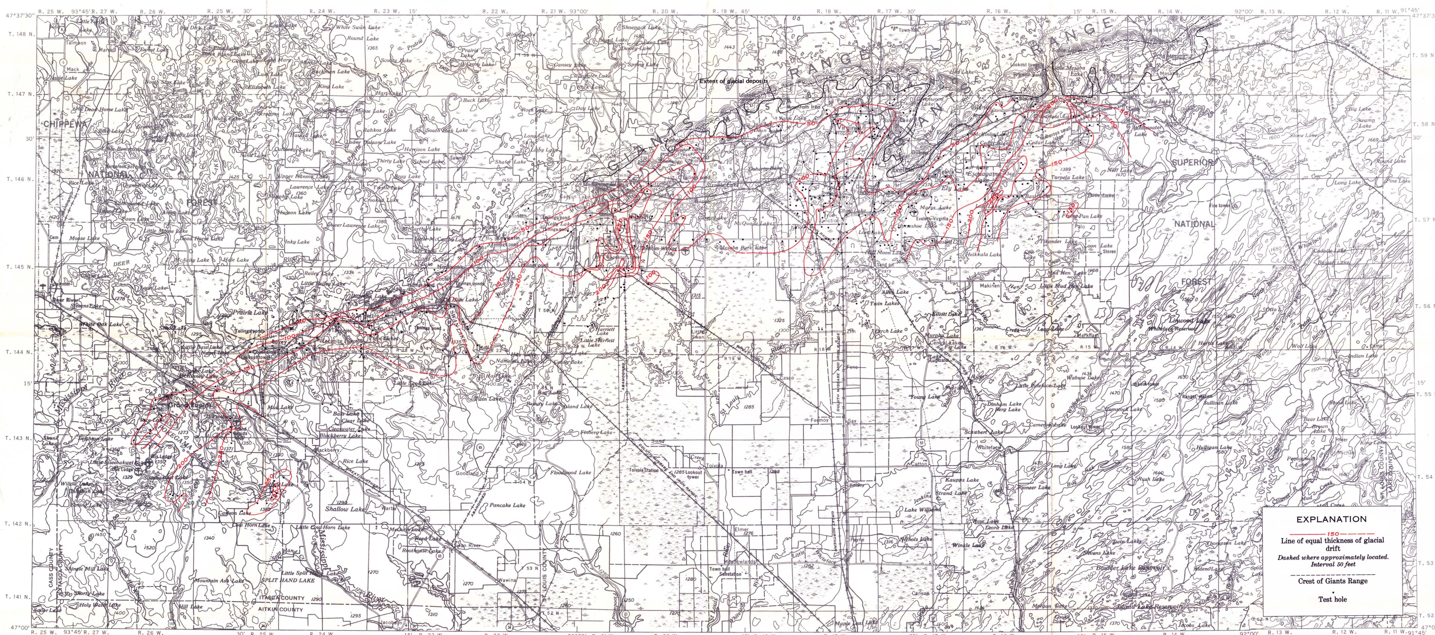
B. THICKNESS OF GLACIAL DRIFT
