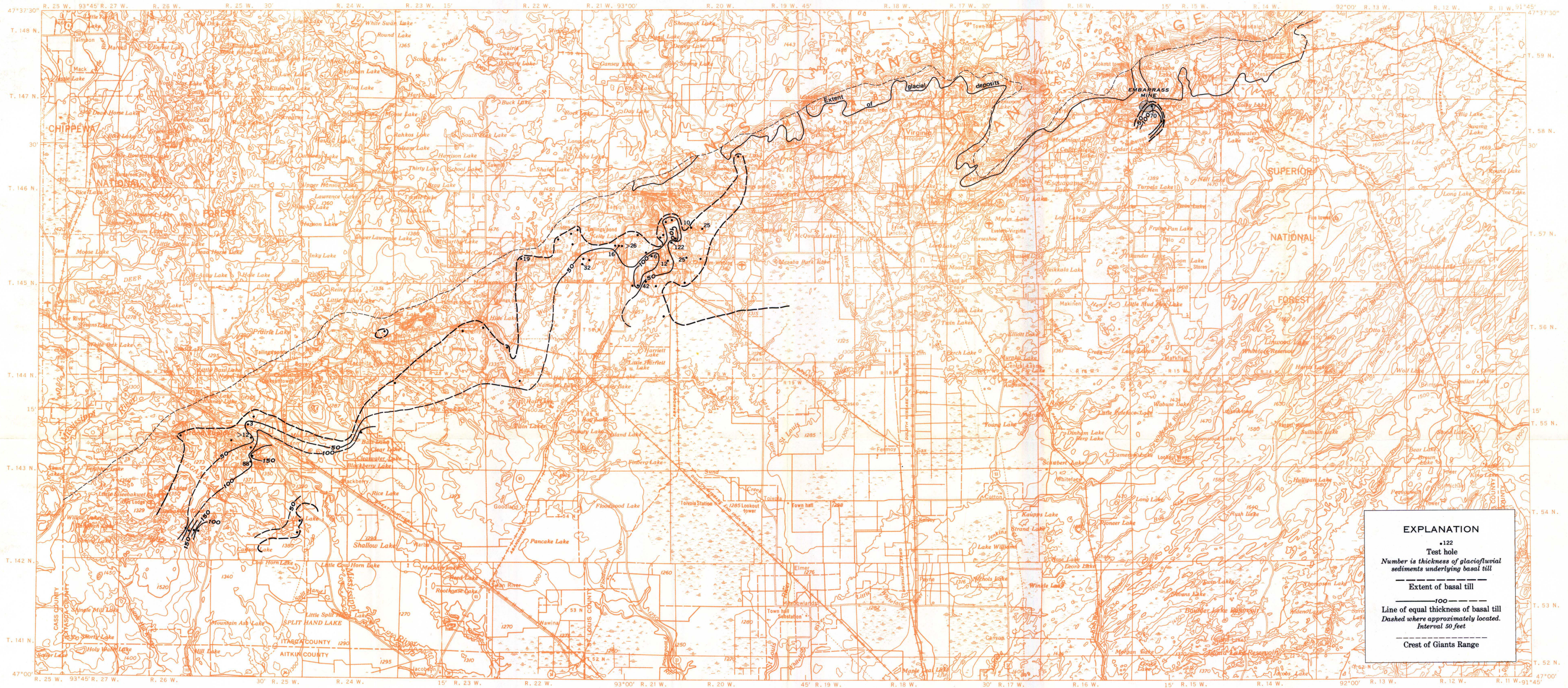
A. EXTENT AND THICKNESS OF BASAL TILL
