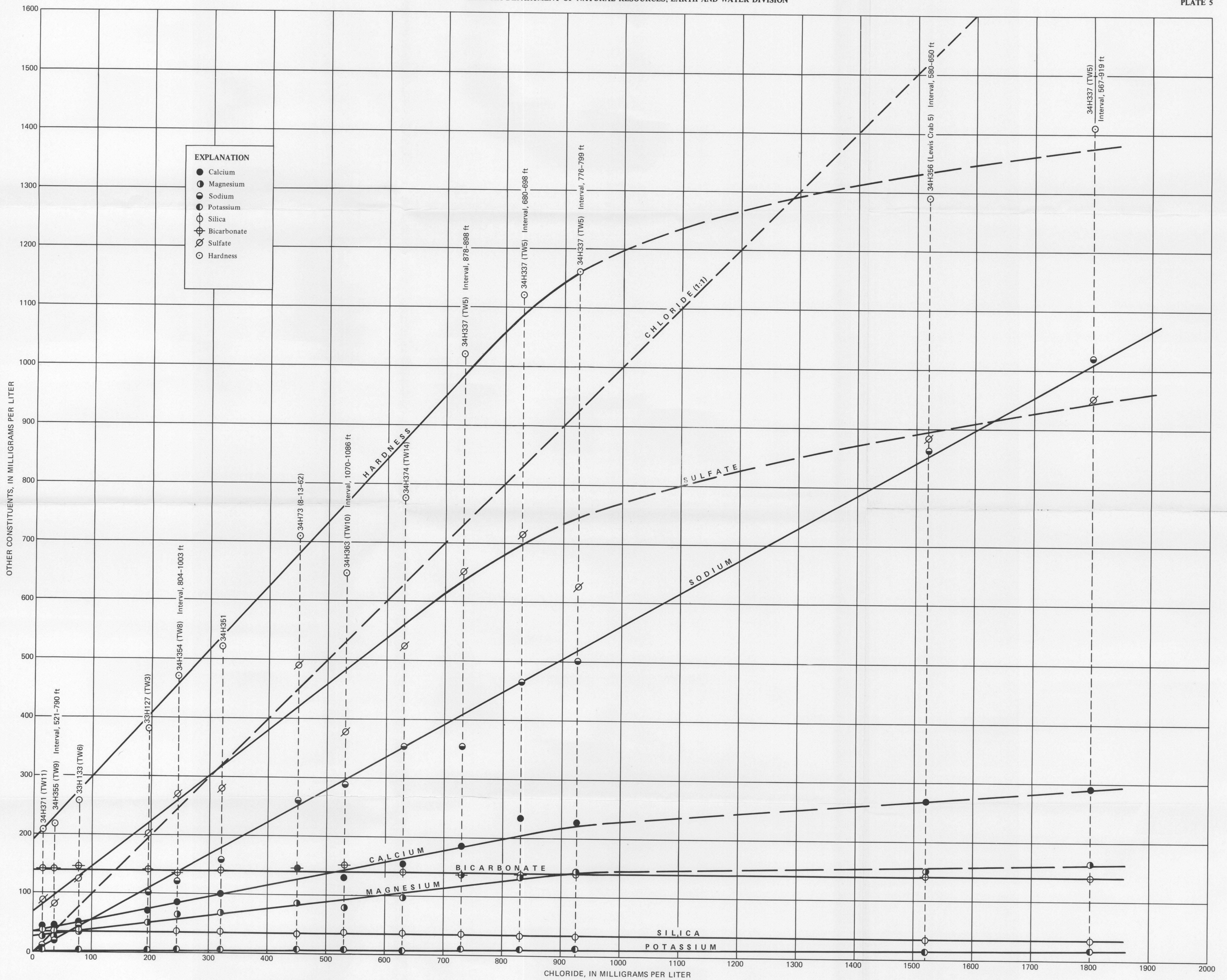
GRAPH SHOWING ION CONCENTRATIONS IN WATER FROM THE PRINCIPAL ARTESIAN AQUIFER, GLYNN COUNTY, GEORGIA
