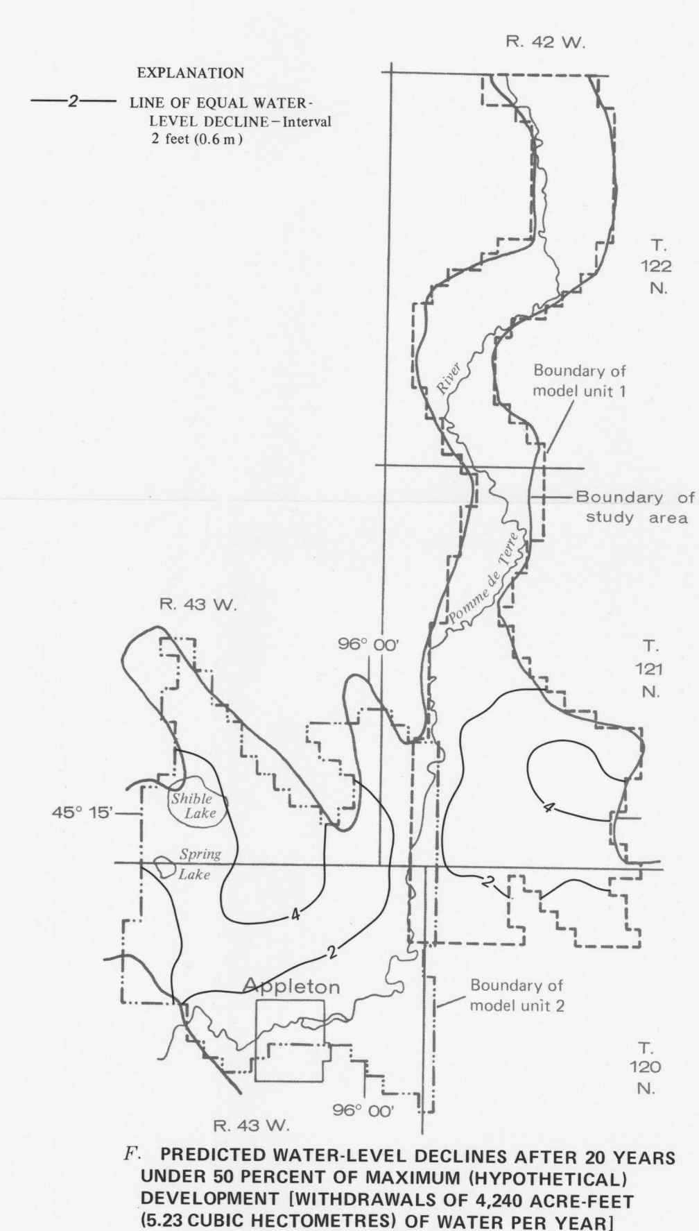
MAPS SHOWING MATHEMATICAL-MODEL ANALYSIS OF SURFICIAL OUTWASH AQUIFER, APPLETON AREA, MINNESOTA
