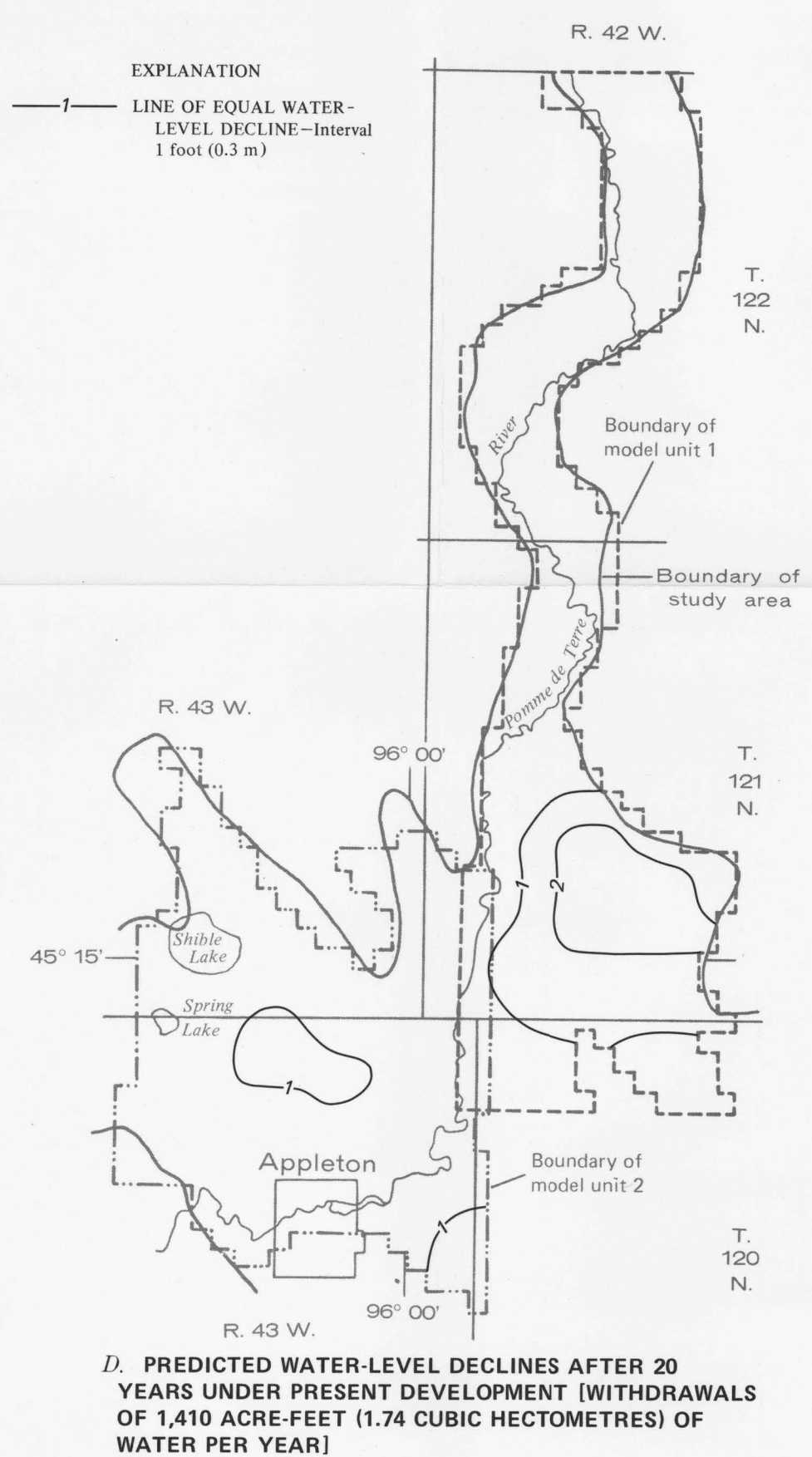
MAPS SHOWING MATHEMATICAL-MODEL ANALYSIS OF SURFICIAL OUTWASH AQUIFER, APPLETON AREA, MINNESOTA
