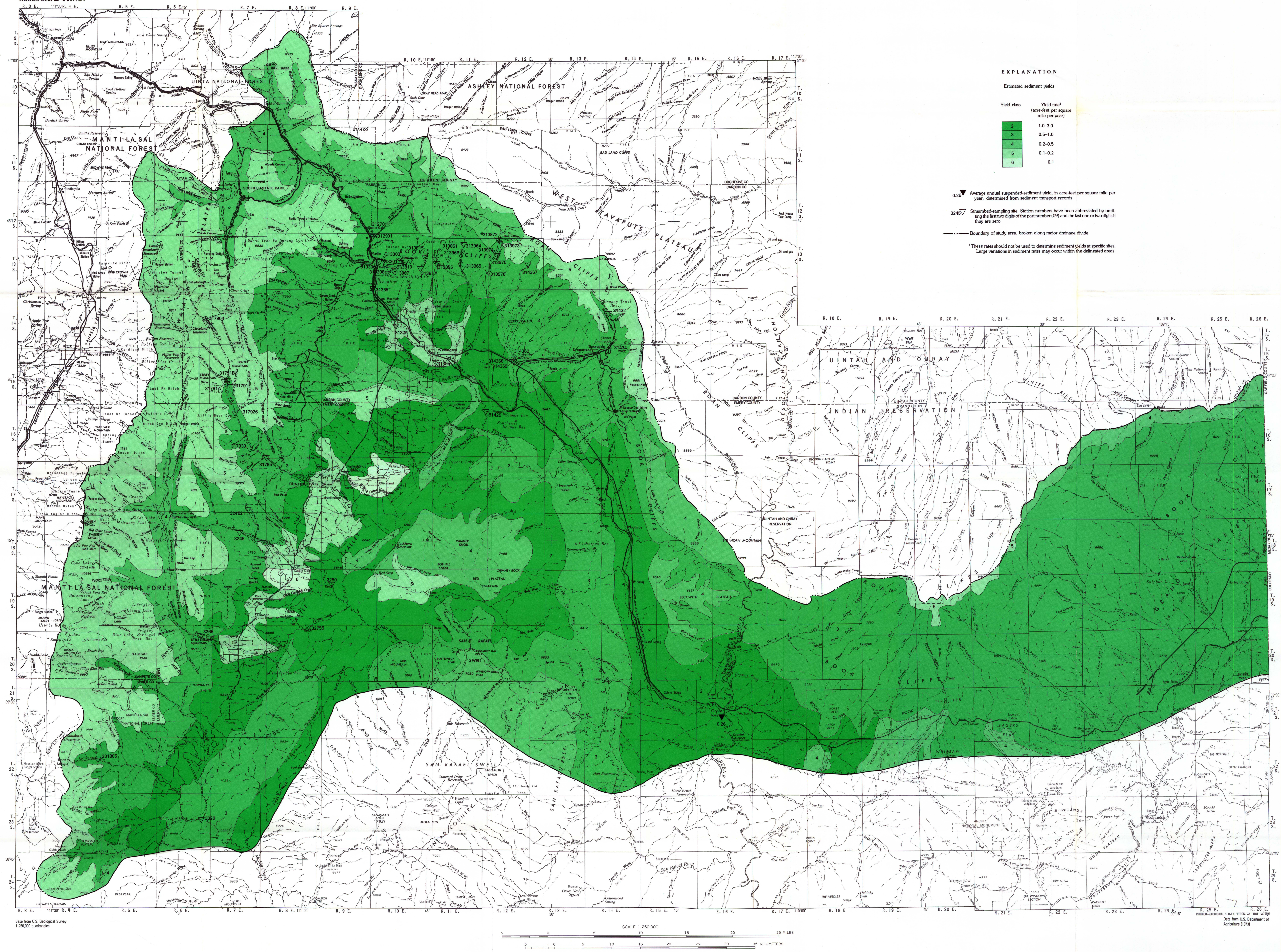
MAP SHOWING ESTIMATED SEDIMENT YIELDS, WASATCH PLATEAU-BOOK CLIFFS COAL-FIELDS AREA, UTAH
