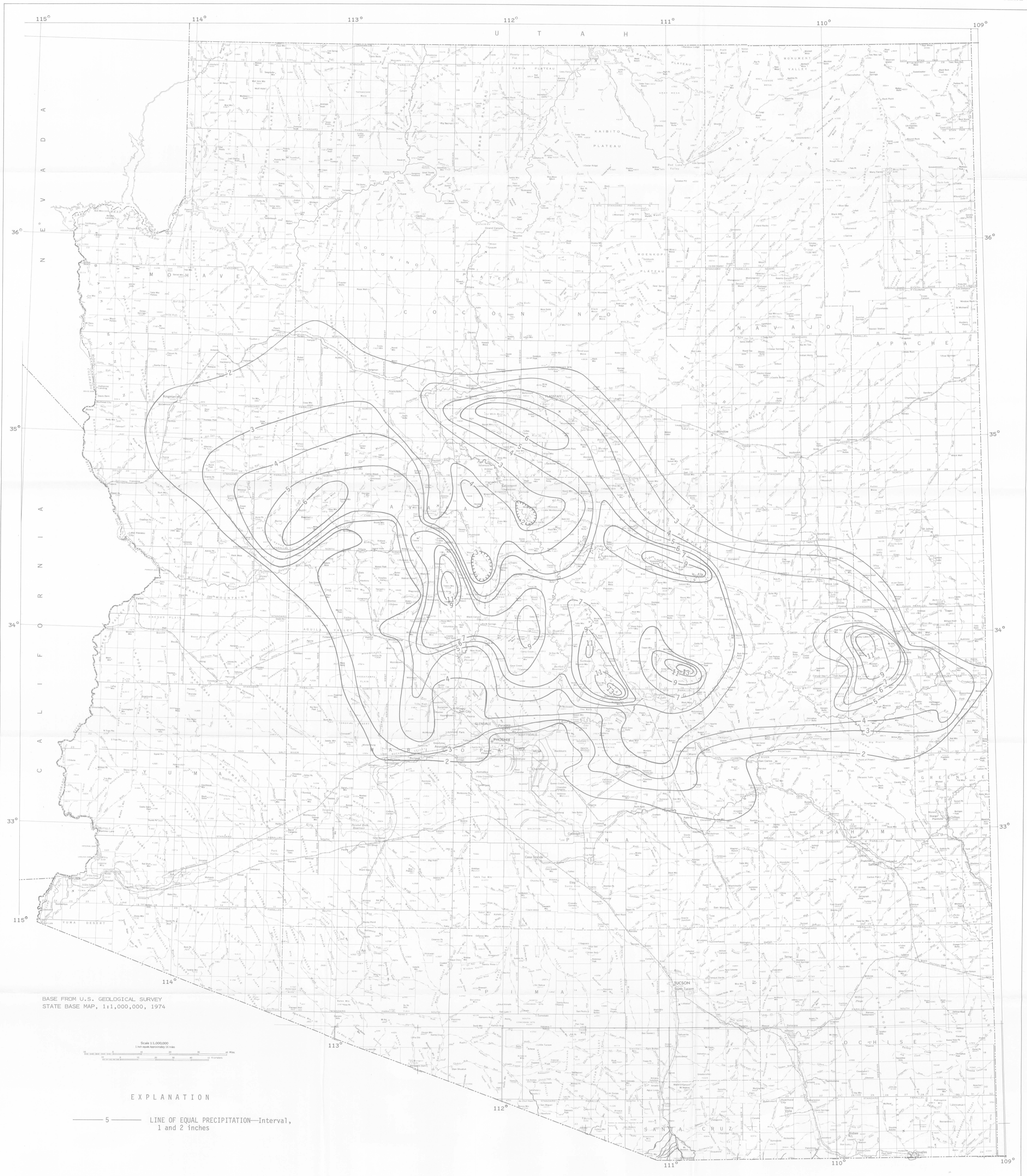
PRECIPITATION IN CENTRAL ARIZONA, FEBRUARY 27 TO MARCH 3, 1978
