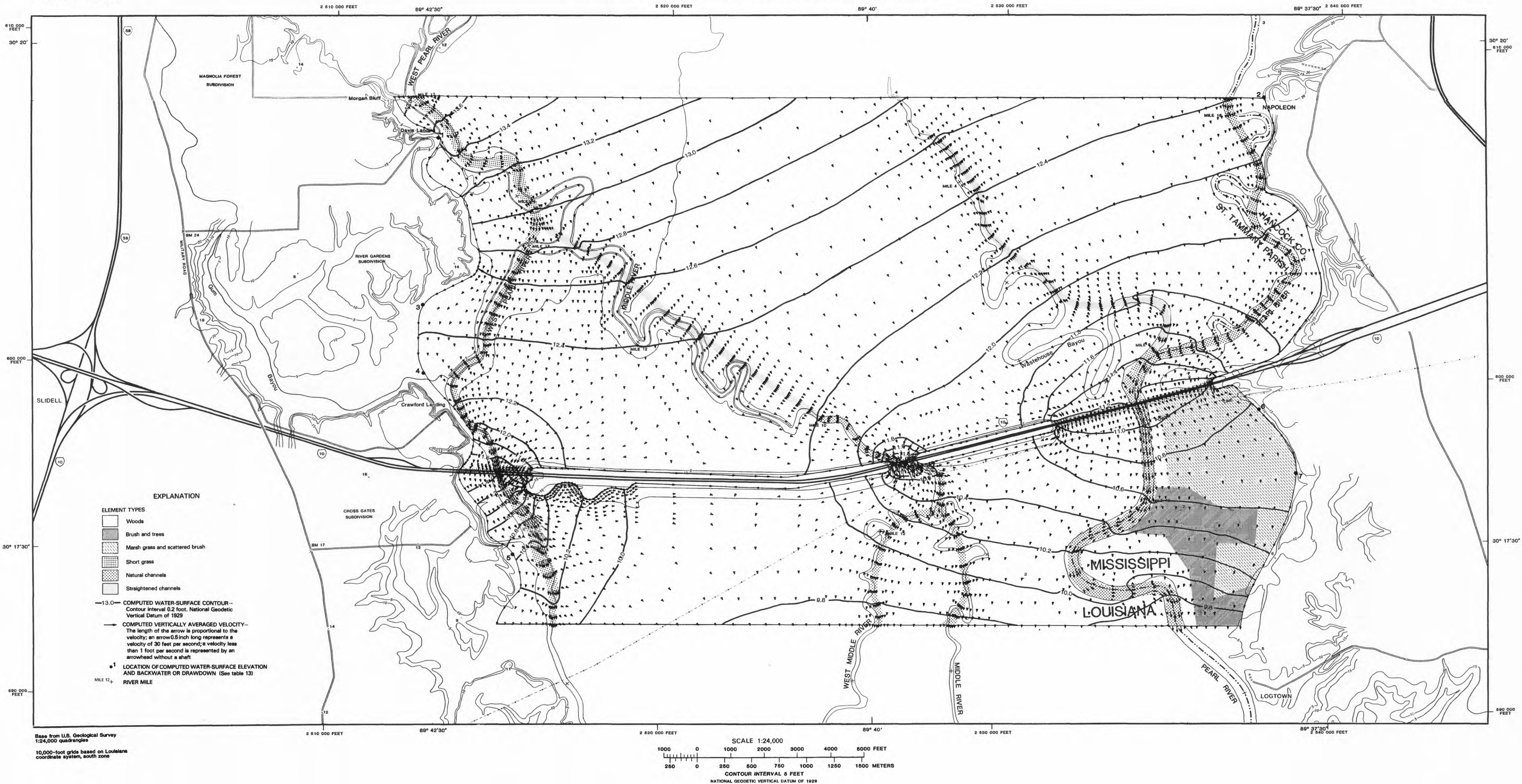
COMPUTED WATER-SURFACE CONTOURS AND VELOCITY FIELD FOR ALTERNATIVE 1
