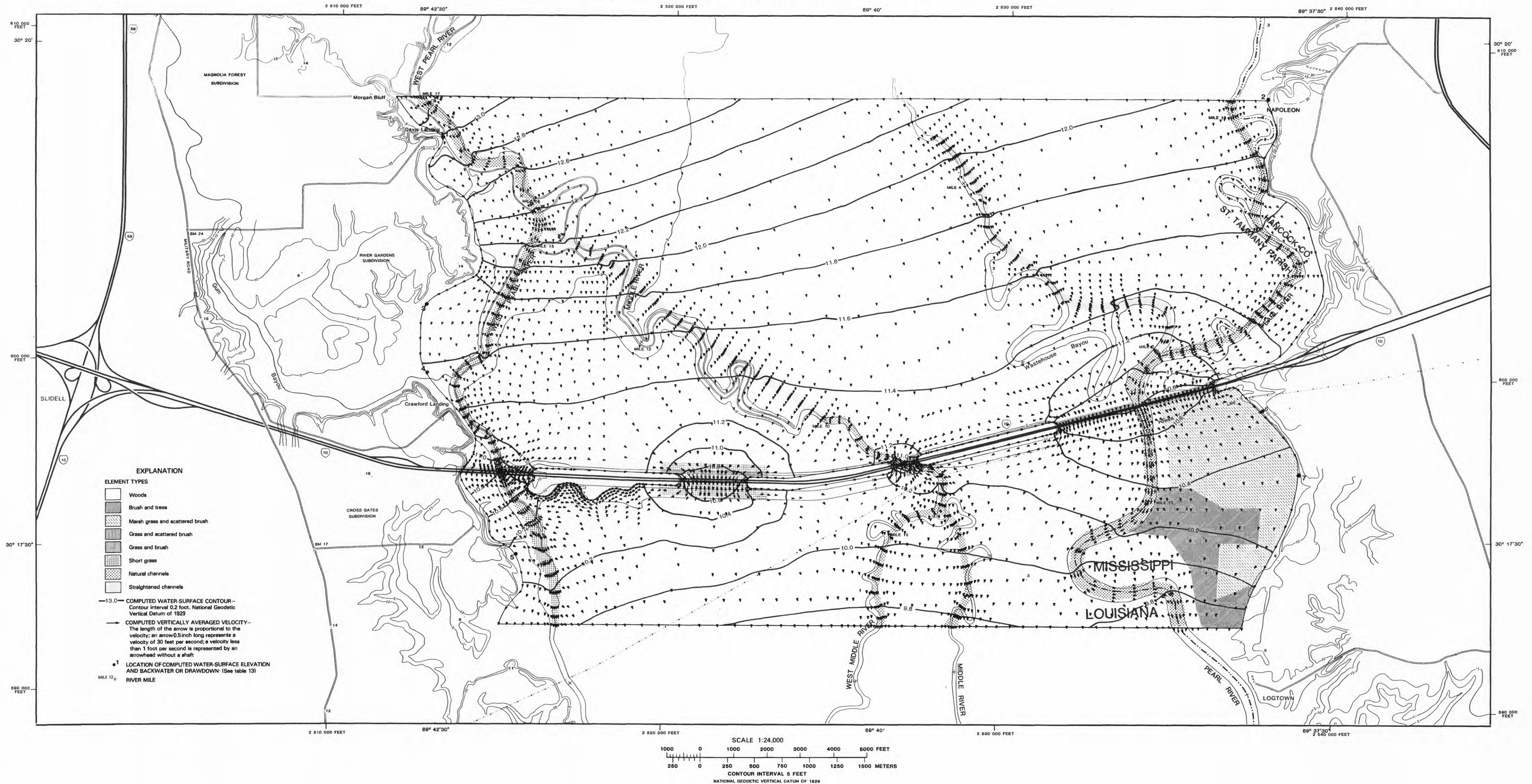
COMPUTED WATER-SURFACE CONTOURS AND VELOCITY FIELD FOR ALTERNATIVE 2
