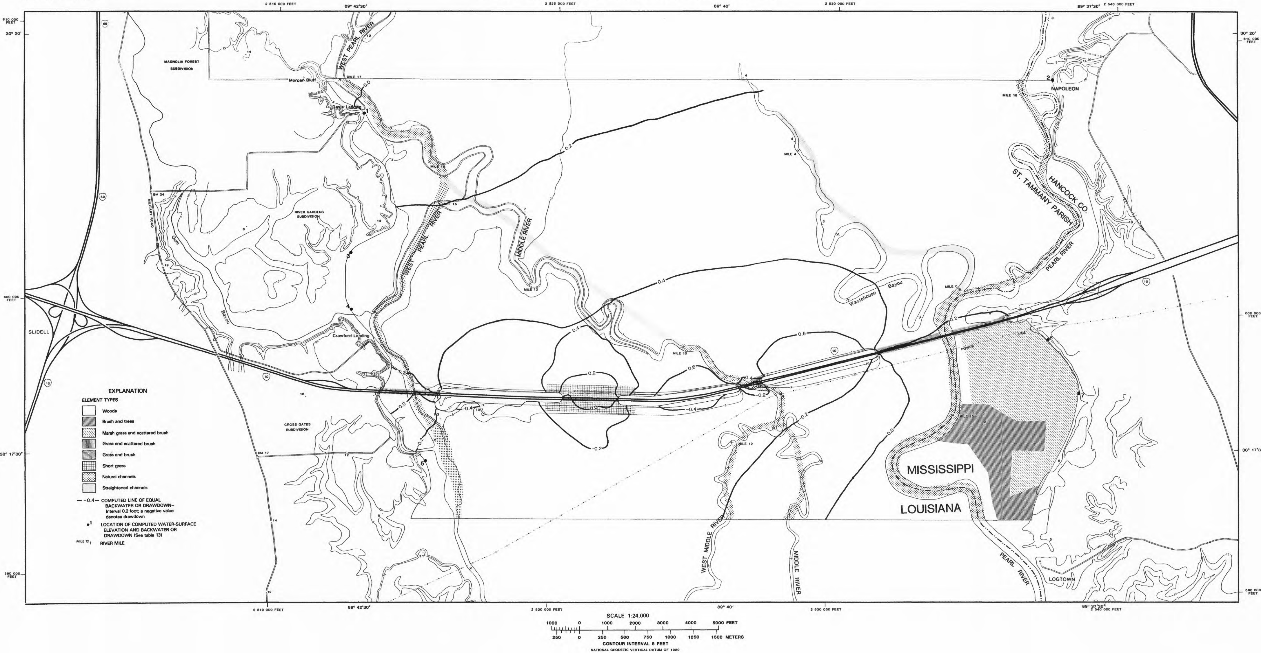
COMPUTED LINE OF EQUAL BACKWATER AND DRAWDOWN FOR ALTERNATIVE 2
