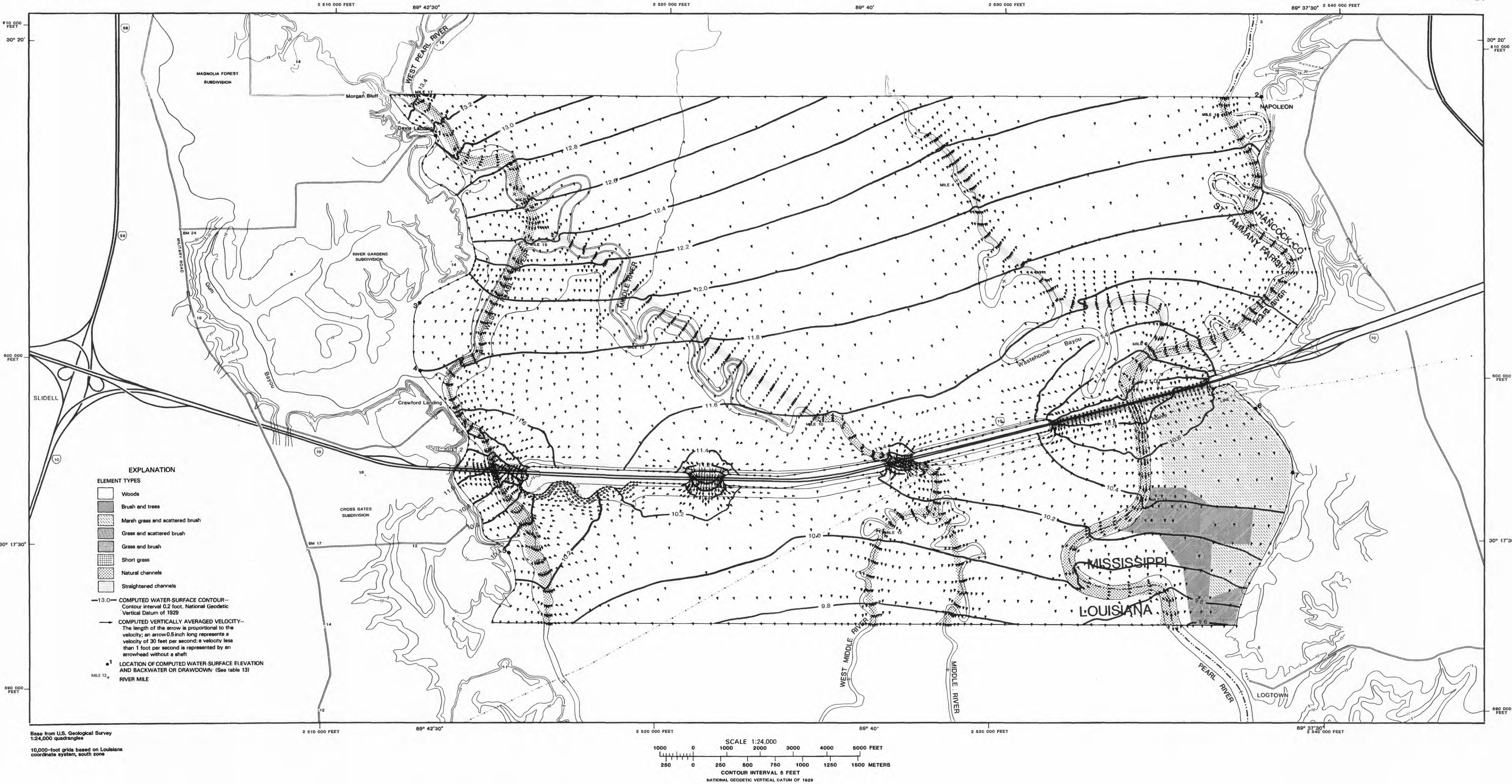
COMPUTED WATER-SURFACE CONTOURS AND VELOCITY FIELD FOR ALTERNATIVE 4
