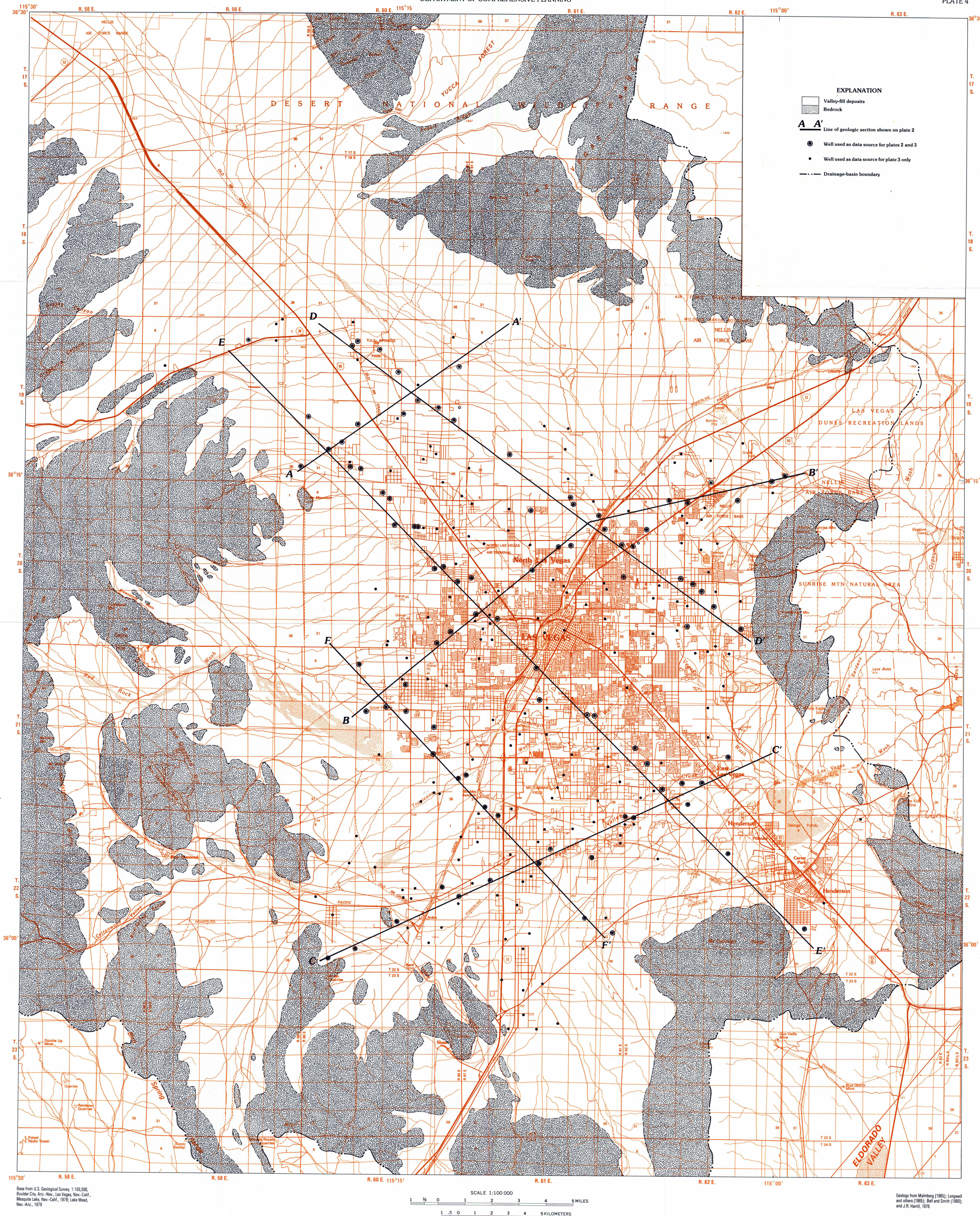
INDEX MAP SHOWING LOCATIONS OF GEOLOGIC SECTIONS ON PLATE 2 AND WELLS ON PLATES 2 AND 3, LAS VEGAS VALLEY, NEVADA
