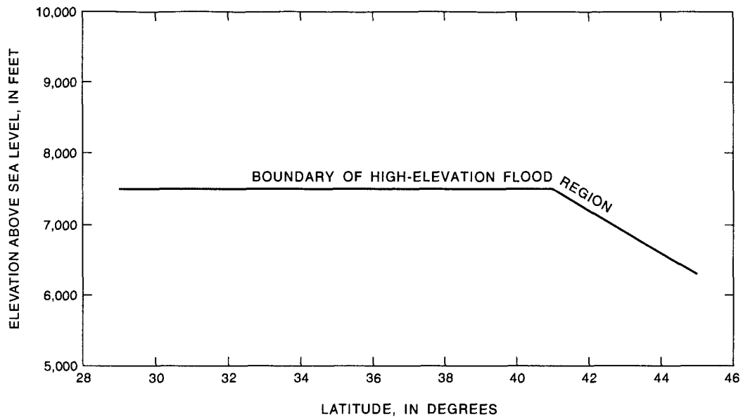
Figure 5. Estimated elevation threshold for large floods caused by thunderstorms in the southwestern United States.
