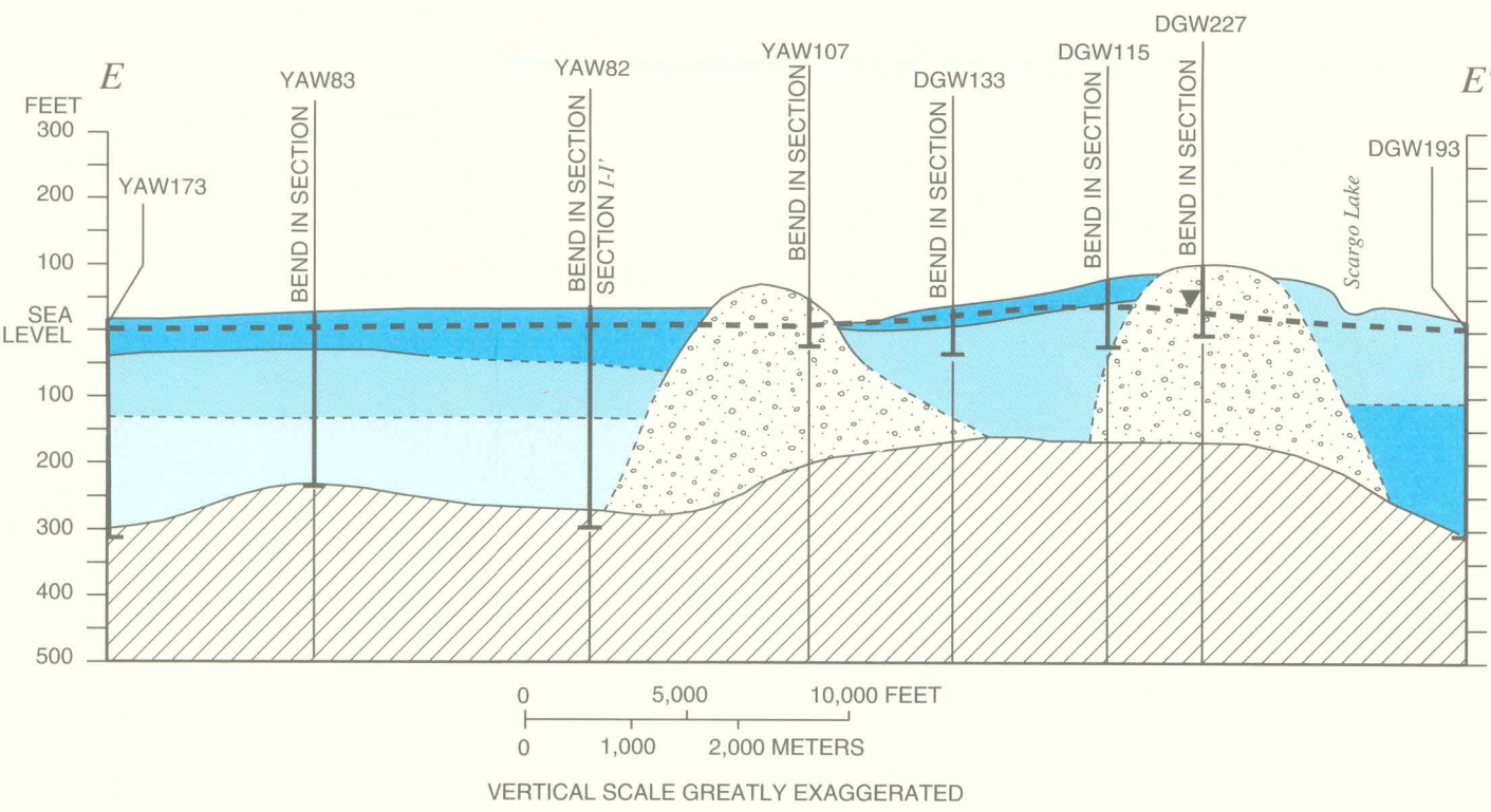
E. Hydrogeologic section E-E'
