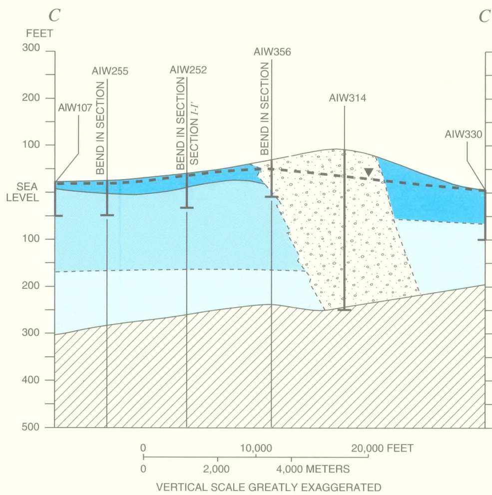
C. Hydrogeologic section C-C'
