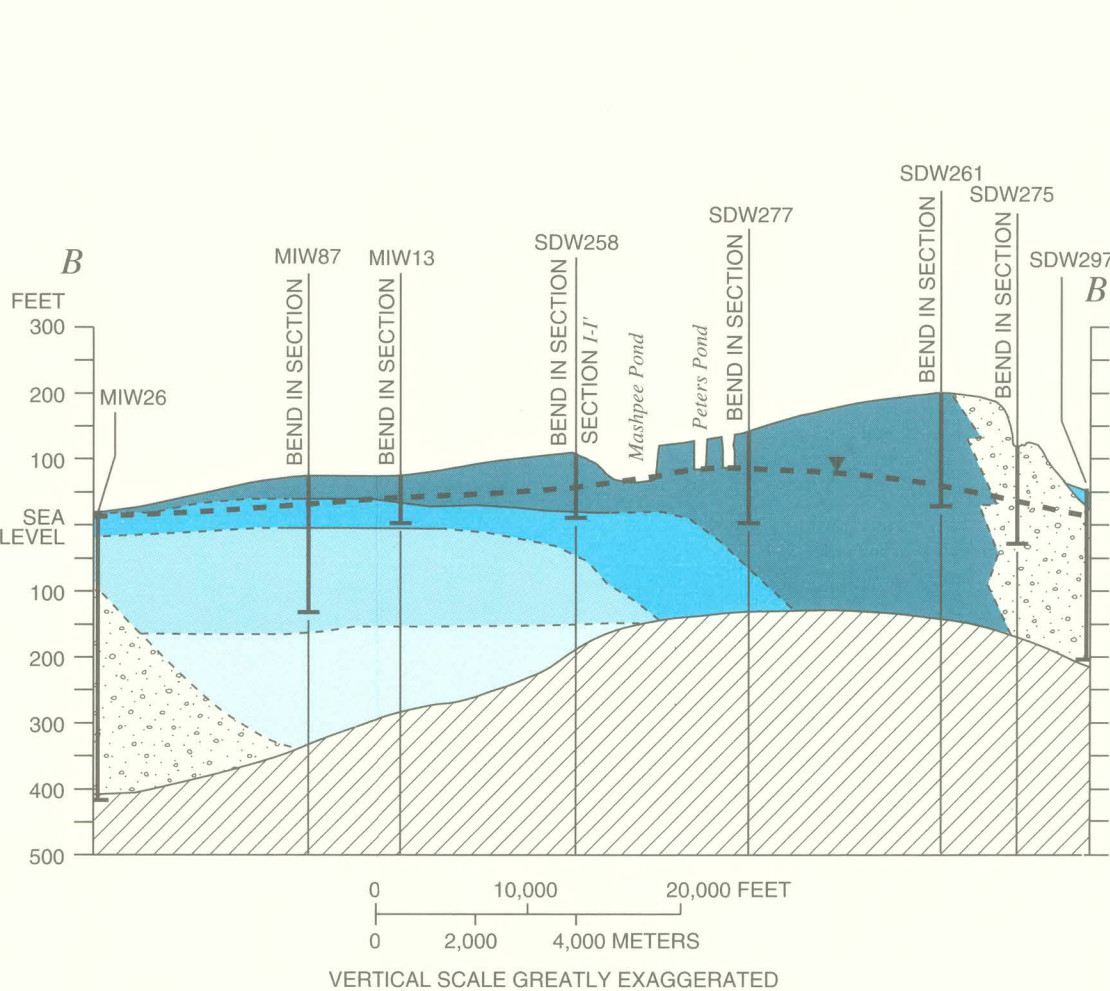
B. Hydrogeologic section B-B'
