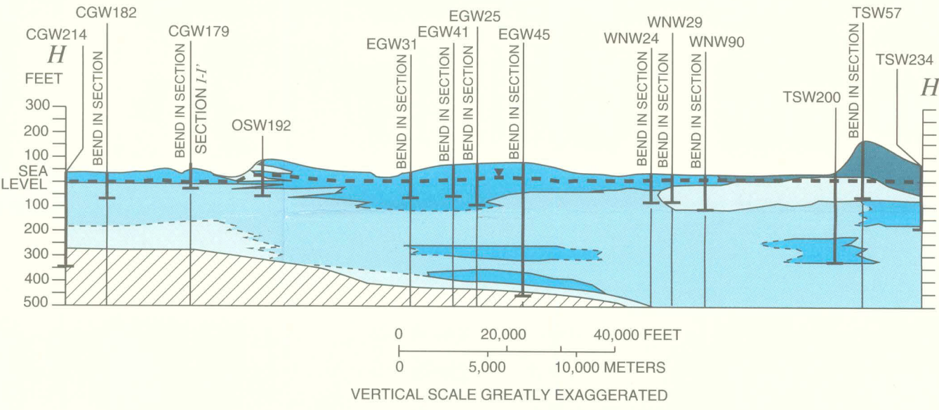
H. Hydrogeologic section H-H'
