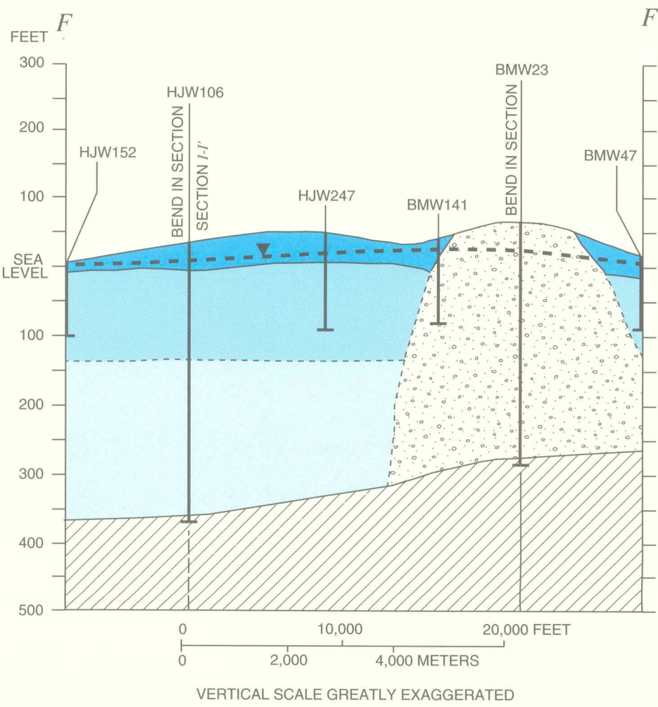
F. Hydrogeologic section F-F'
