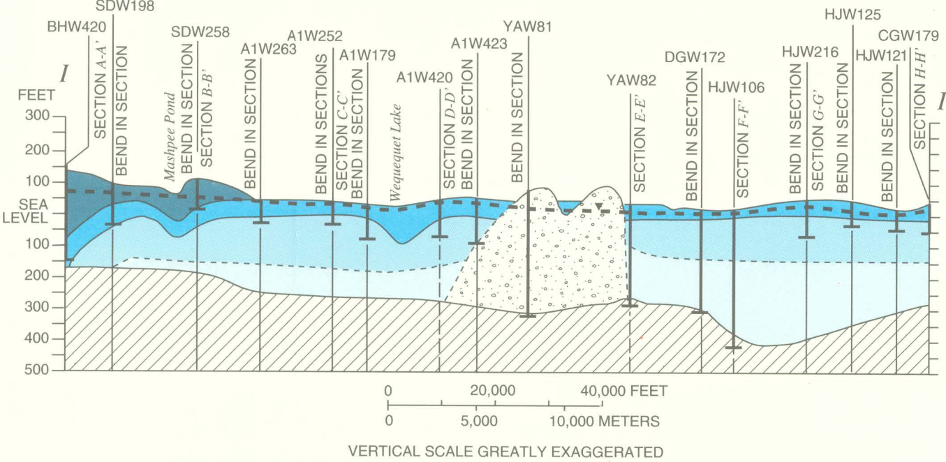
I. Hydrogeologic section I-I'
