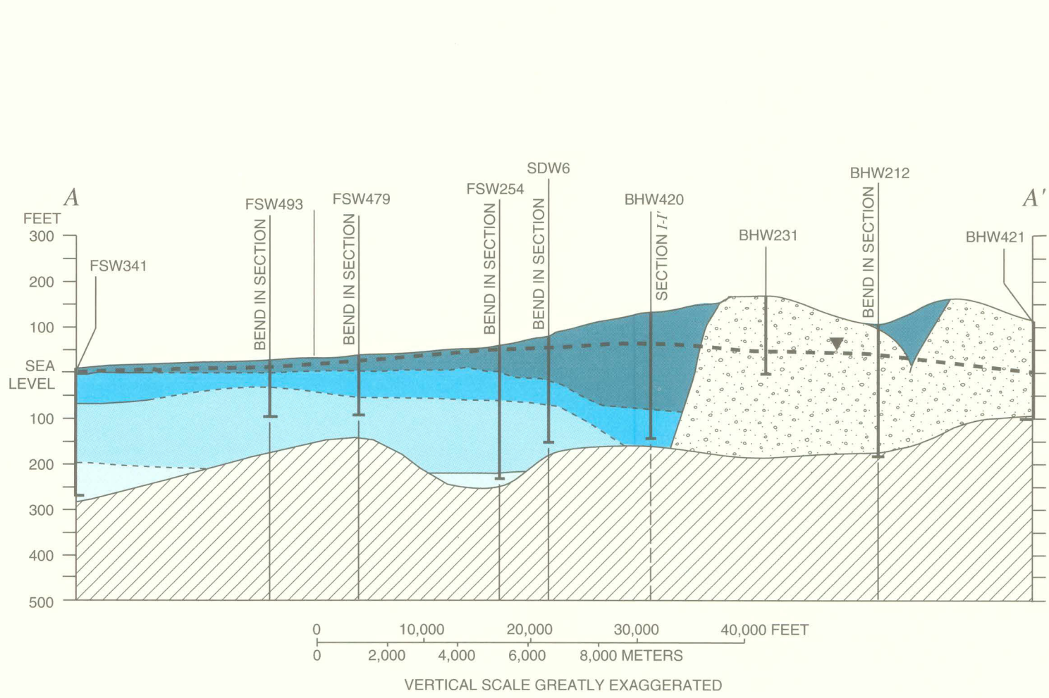
A. Hydrogeologic section A-A'
