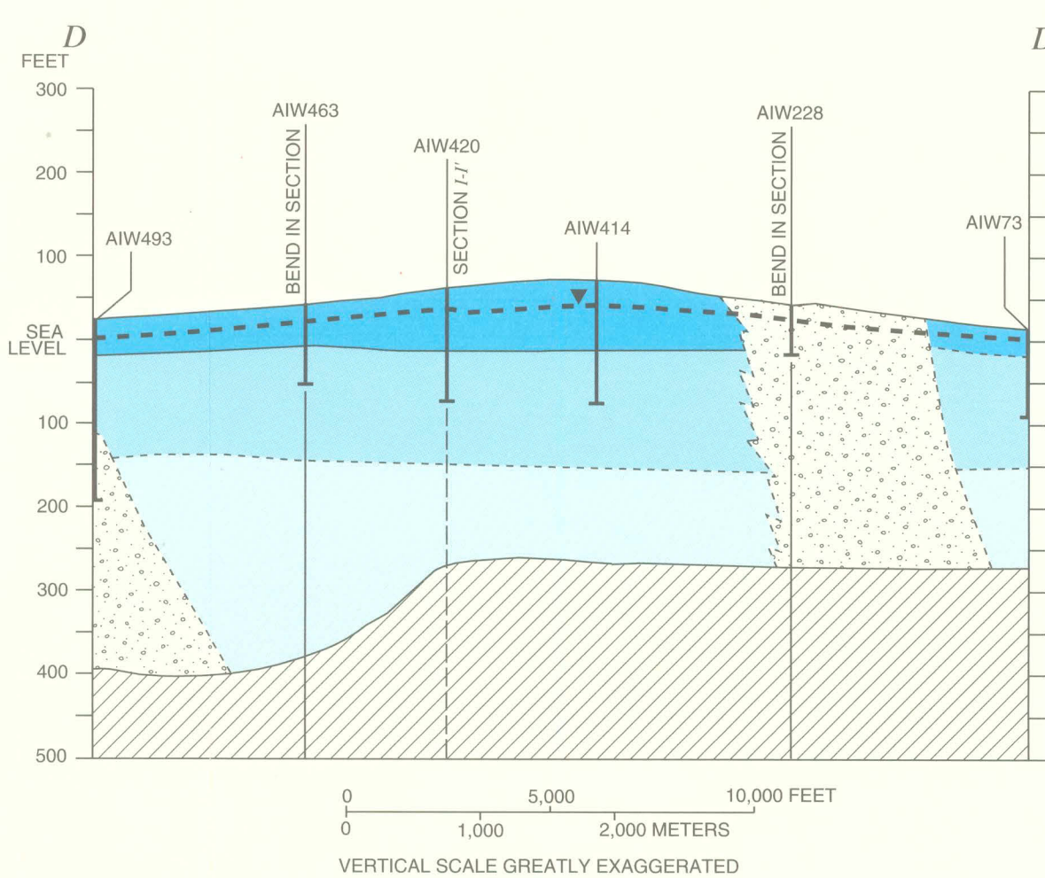
D. Hydrogeologic section D-D'
