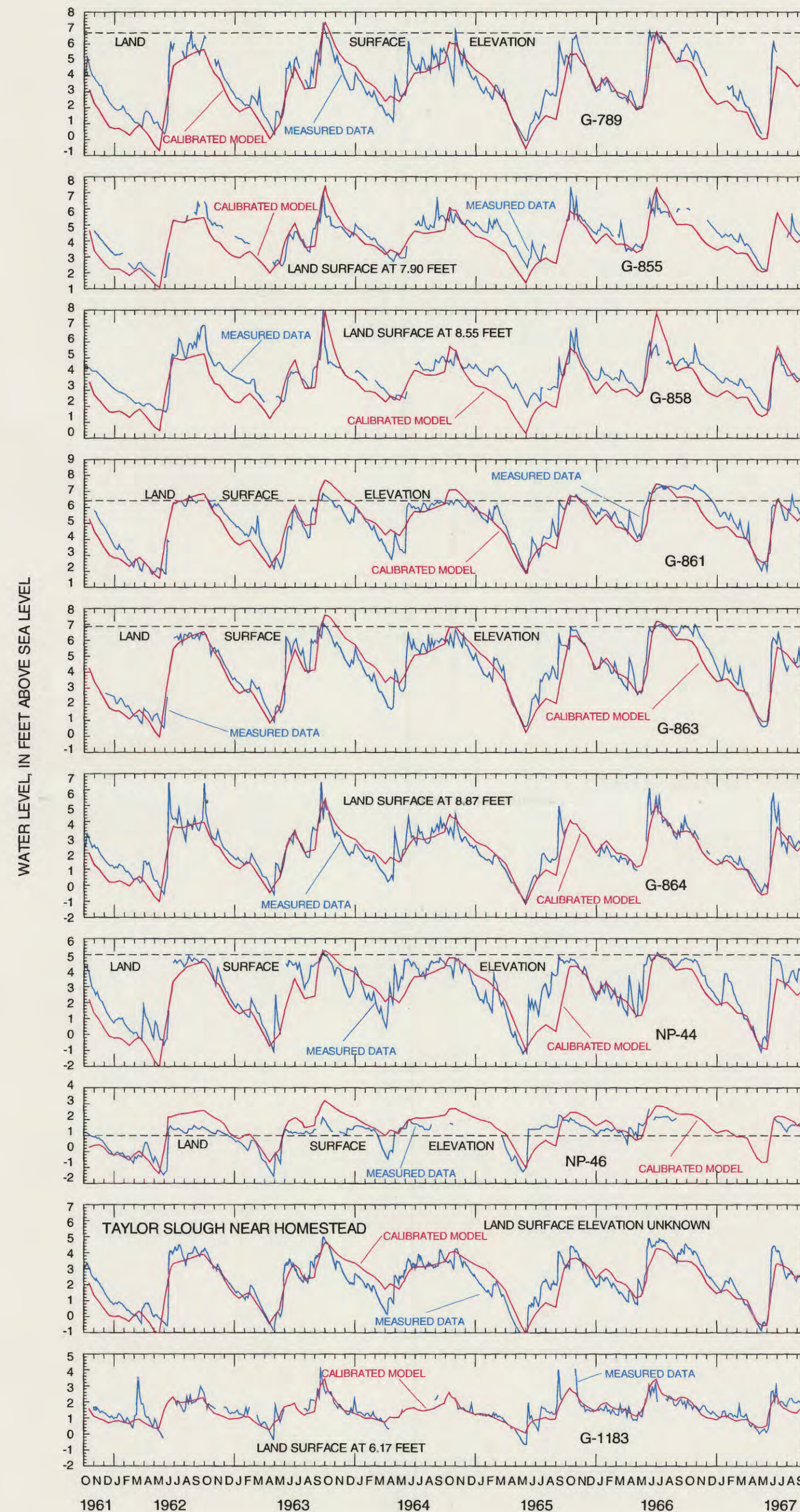
PLATE 3.—COMPARISON HYDROGRAPHS FOR TIME PERIOD 3 (WATER YEARS 1962-67) AND SELECTED SENSITIVITY ANALYSES
