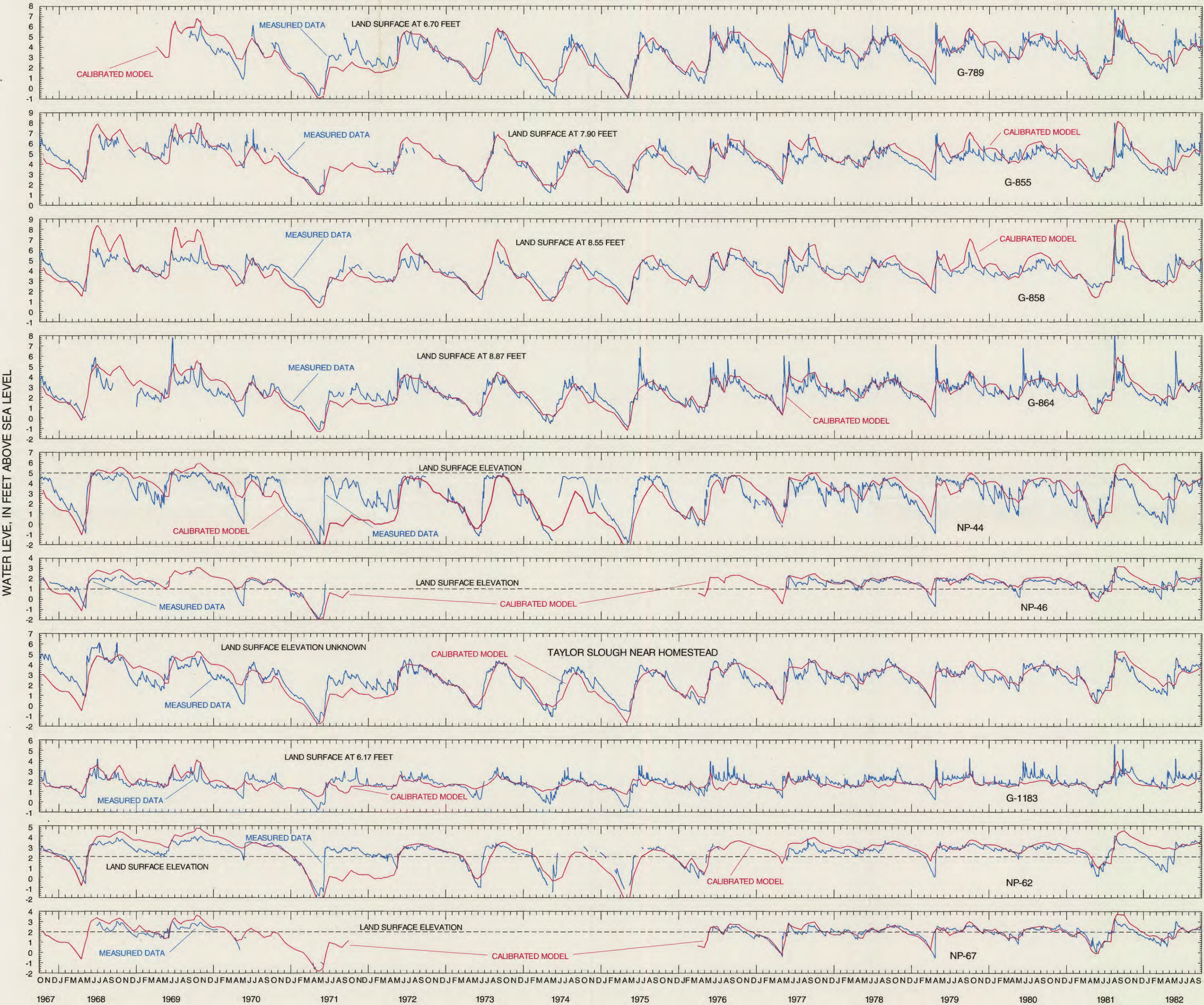
PLATE 5.—COMPARISON HYDROGRAPHS FOR TIME PERIOD 4 (WATER YEARS 1968-82), PART 2
