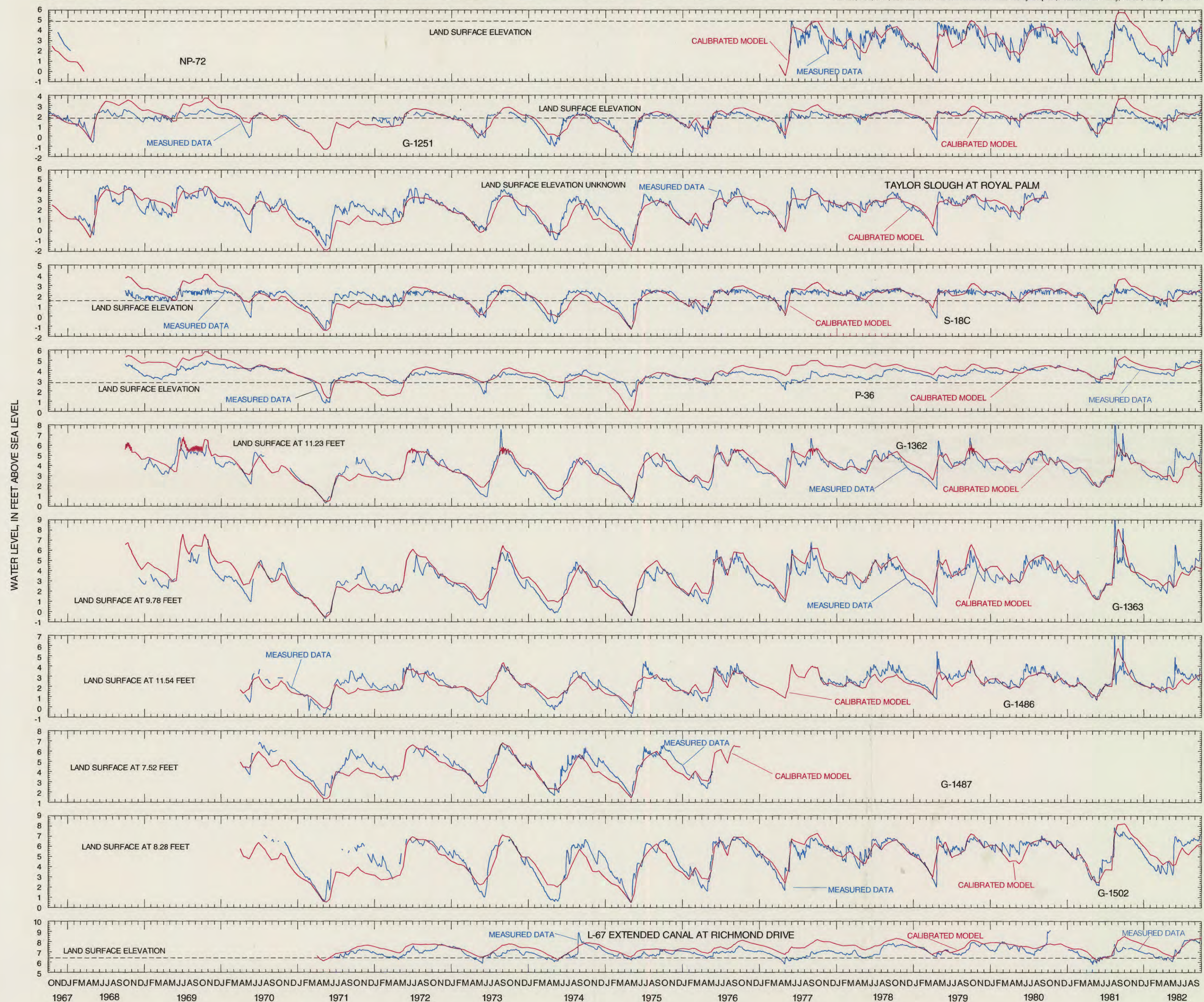
PLATE 6.—COMPARISON HYDROGRAPHS FOR TIME PERIOD 4 (WATER YEARS 1968-82), PART 3
