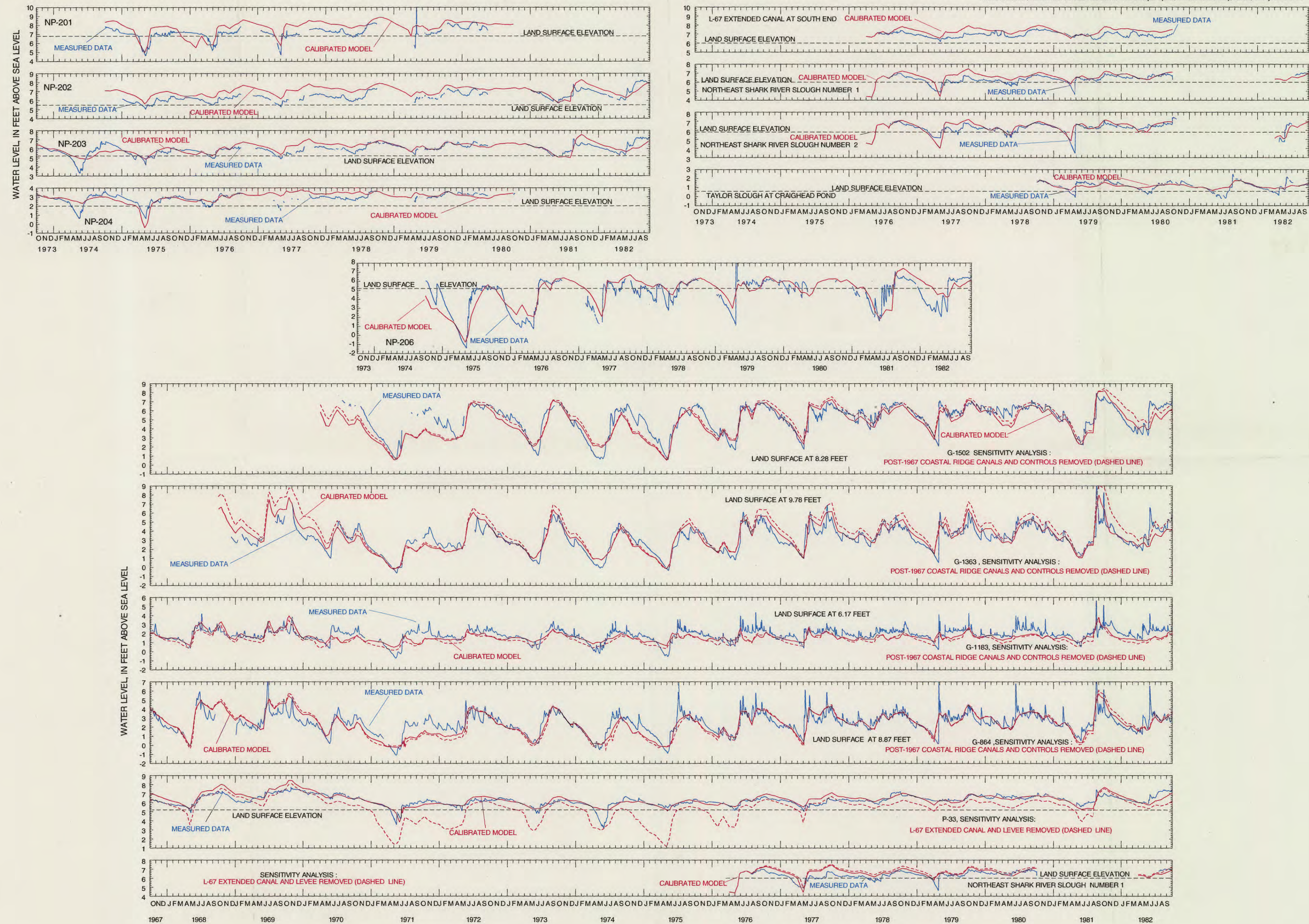
PLATE 7.—COMPARISON HYDROGRAPHS FOR TIME PERIOD 4 (WATER YEARS 1968-82), PART 4, AND SELECTED SENSITIVITY ANALYSES
