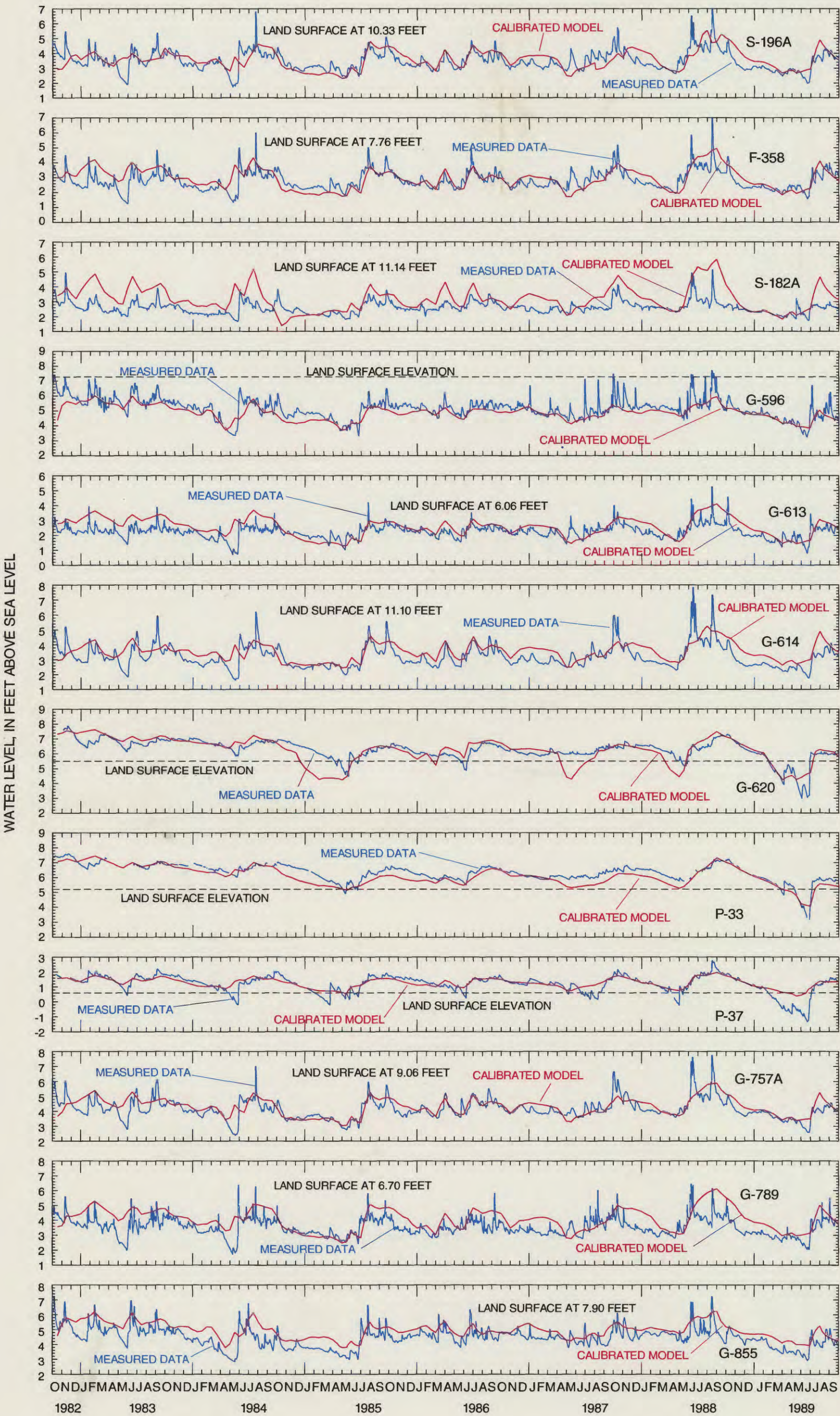
PLATE 8.—COMPARISON HYDROGRAPHS FOR TIME PERIOD 5 (WATER YEARS 1983-89), PART 1
